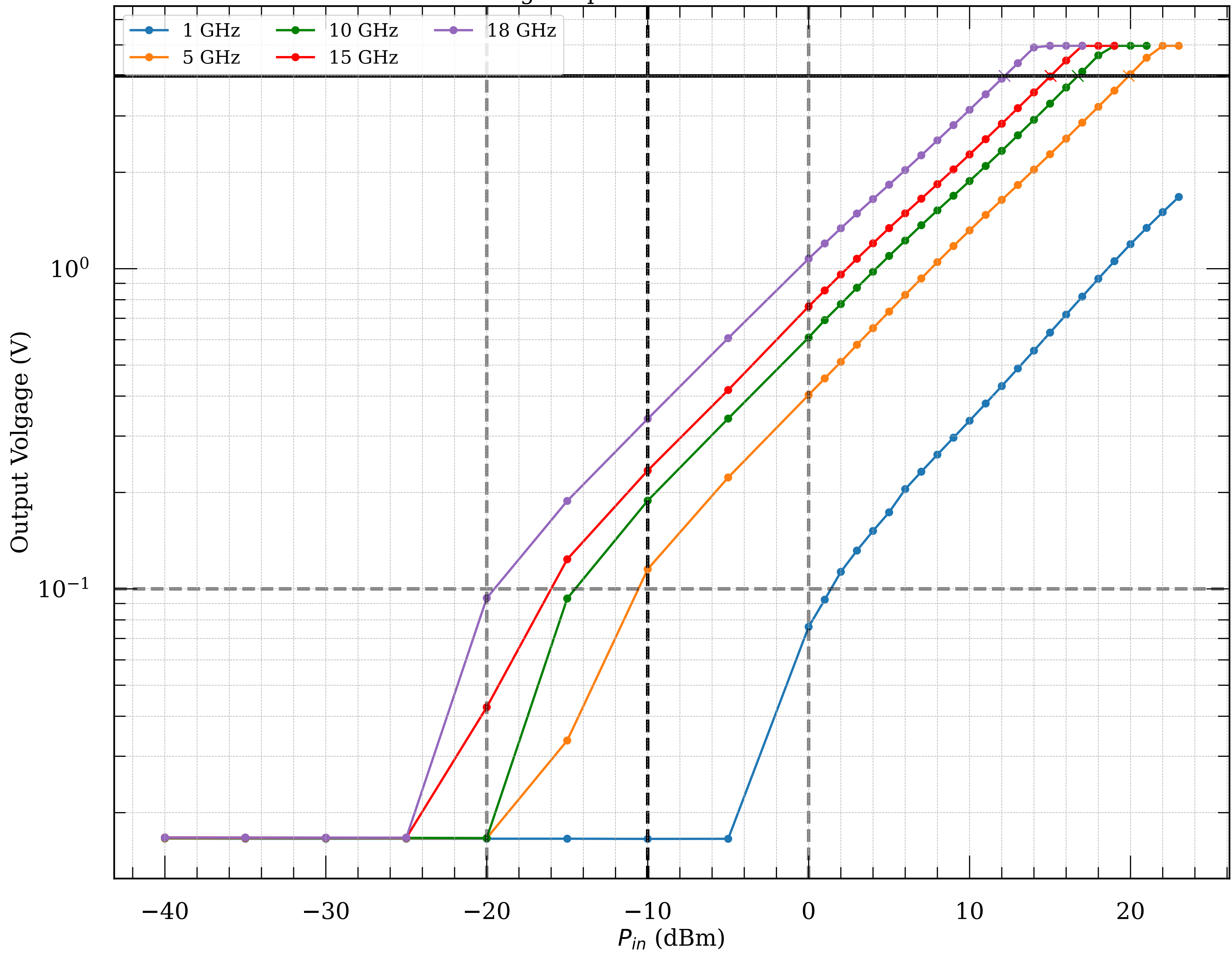
Measured voltage-to-power curve of detector module087
